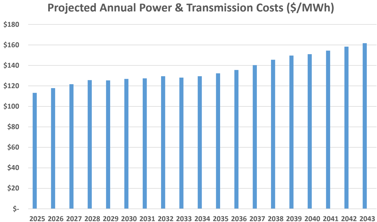
Figure 7-16. Projected annual power and transmission costs per MWh.
