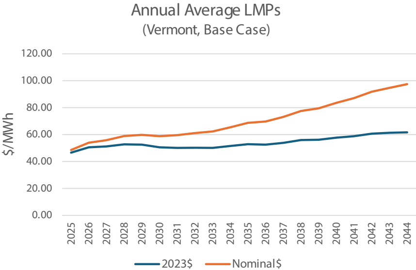
Figure 7-18. Projected Annual Average Energy Market Prices.
