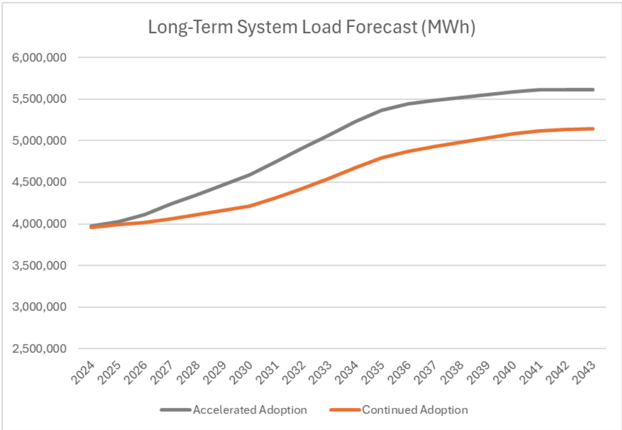
Figure 2-21. Long-term forecasted system load, in annual MWh under each scenario, through 2043, excluding GlobalFoundries.
