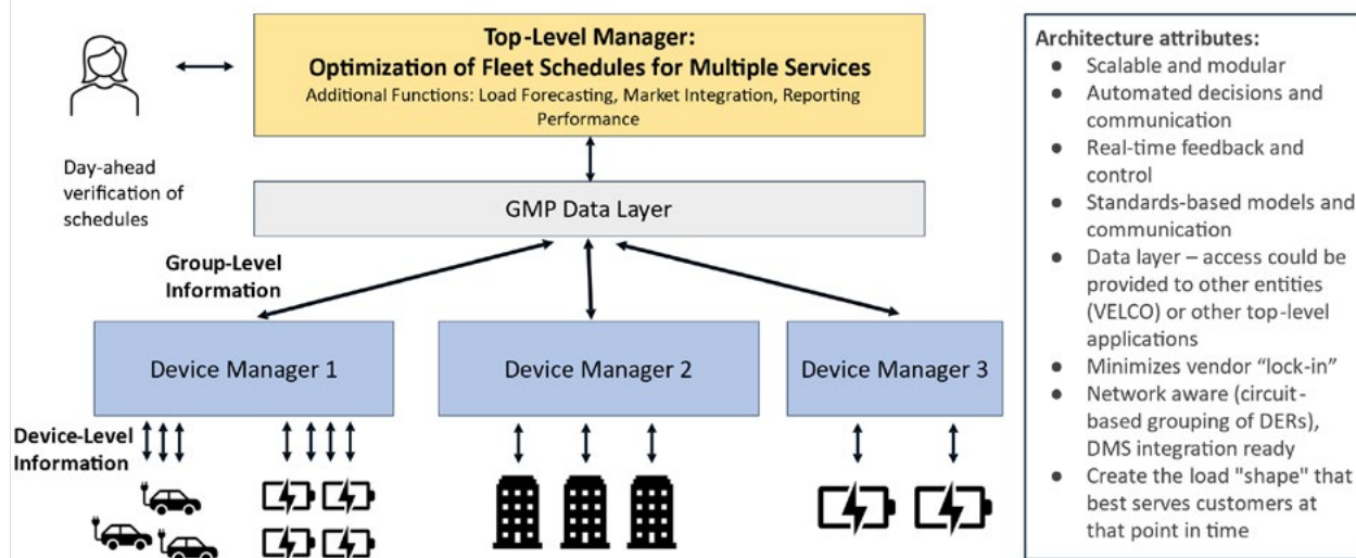
Figure 1-2. GMP's comprehensive strategy for applying DERMS to manage GMP data and relevant devices.
