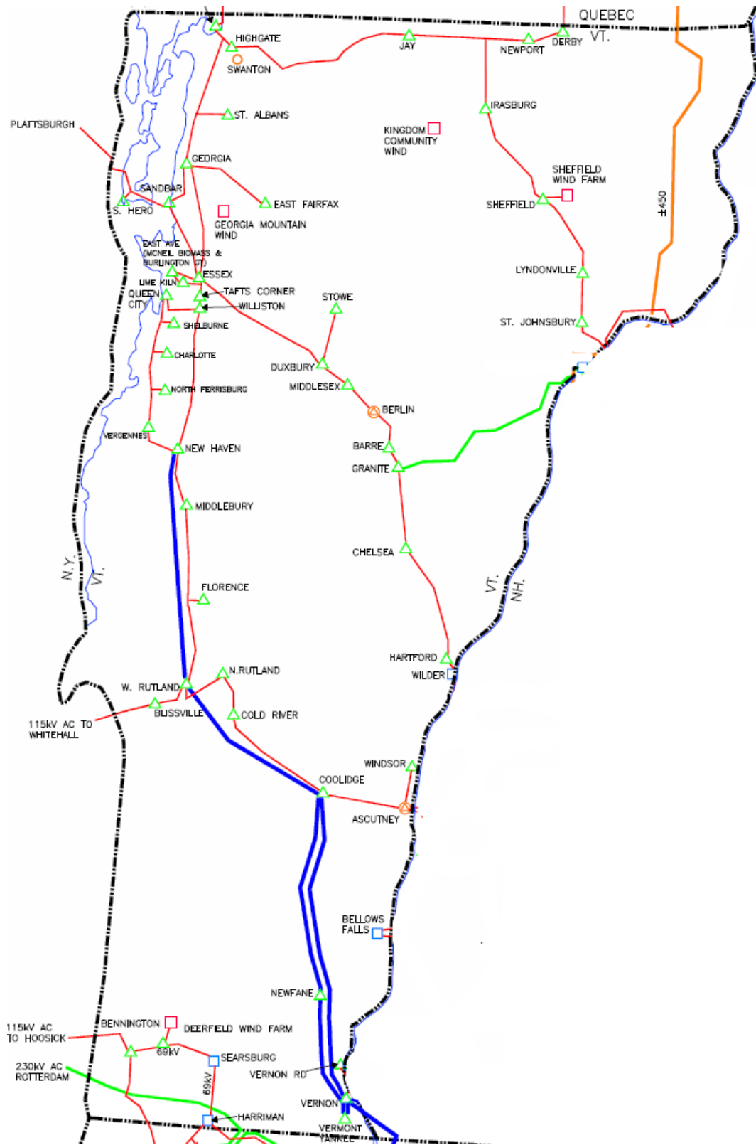
Figure 1-1: Geographic Diagram of the Vermont Area Bulk Electric System
