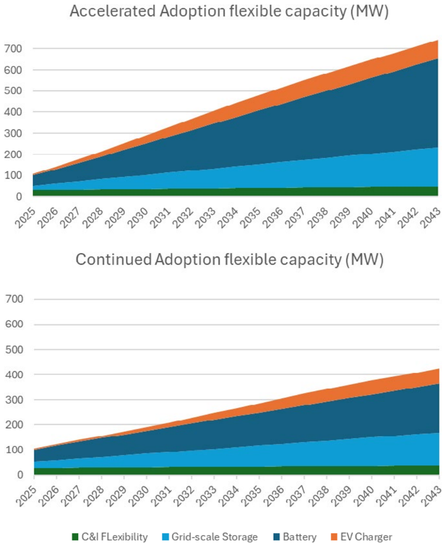
Figure 2-34. Total projected flexible capacity due to EVs, residential energy storage, and other flexible resources through 2043.
