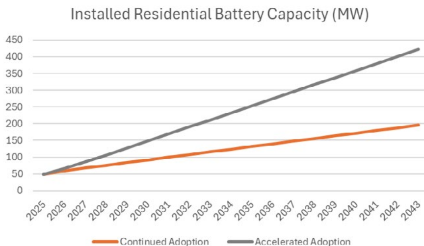
Figure 2-30. Residential installed battery capacity, in MW, through 2043.
