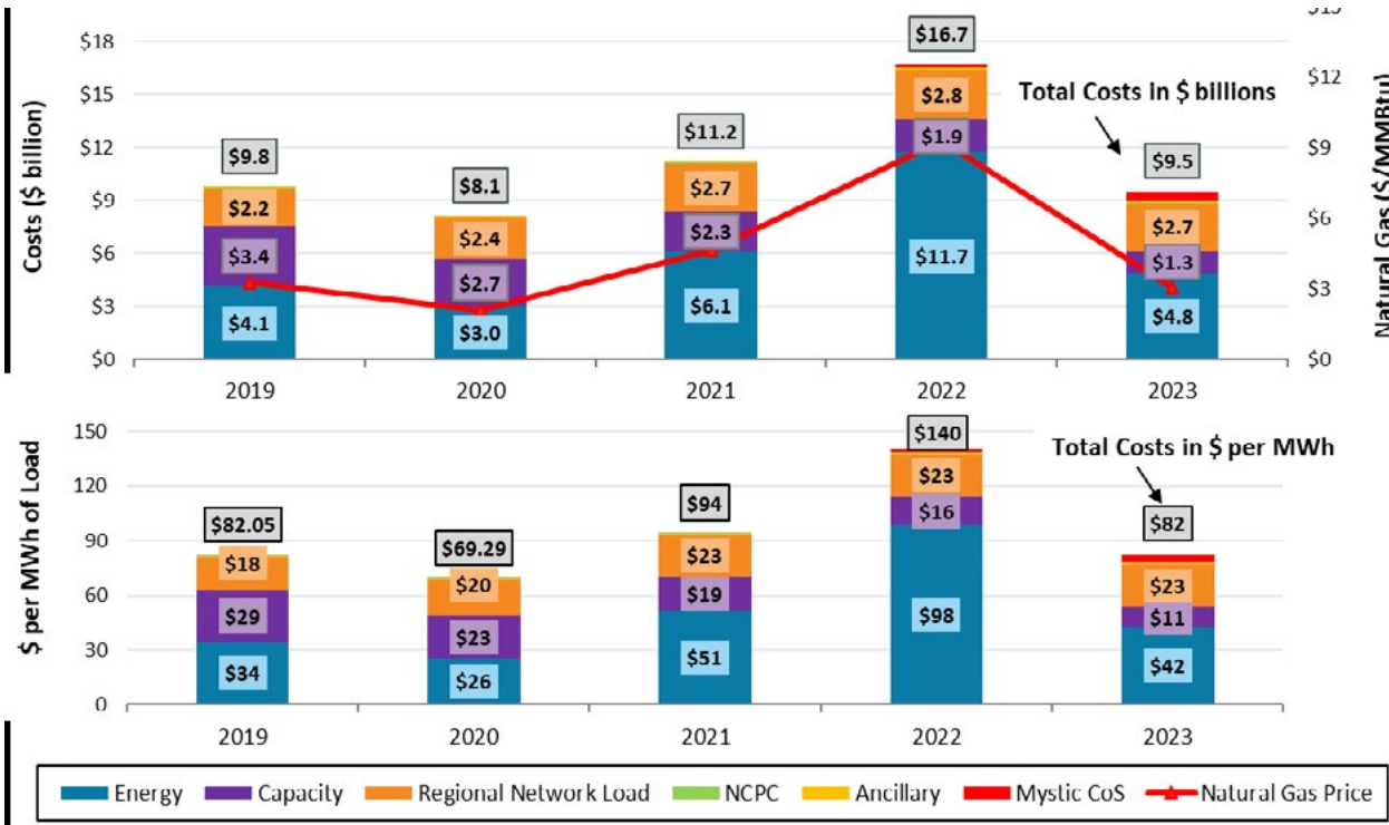
Figure 5-3. Annual value of wholesale electricity markets (Source: ISO New England, IMM Annual Markets Performance Report , Slide 3).
