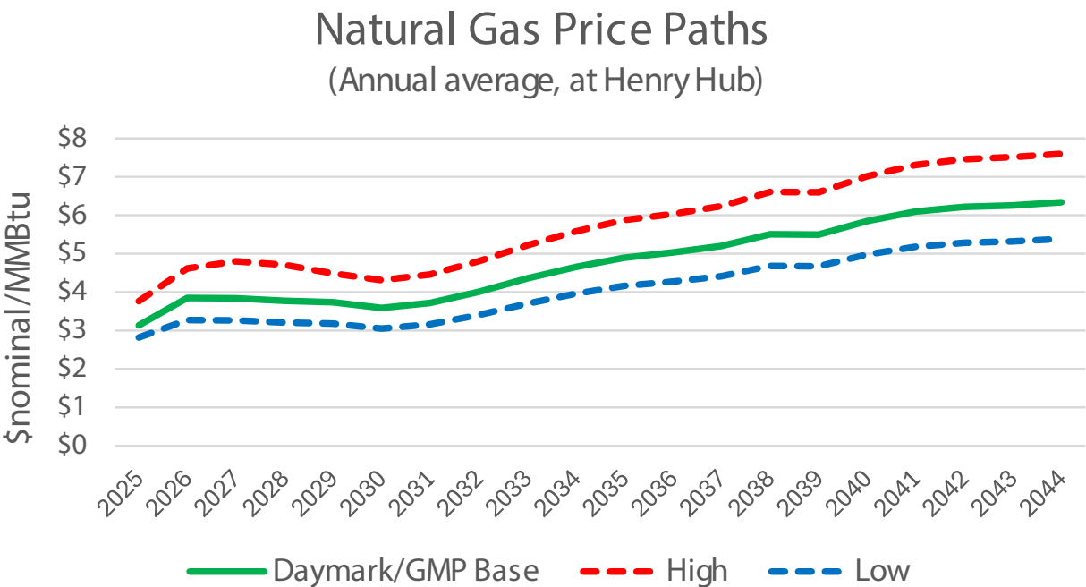
Figure I-6. Natural gas price paths.
